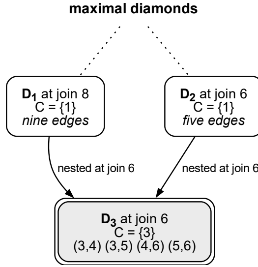
Figure 4.8: Frame 4. The emitted hierarchy of two maximal diamonds, with the inner diamond D_3 stored once and referenced by both.
