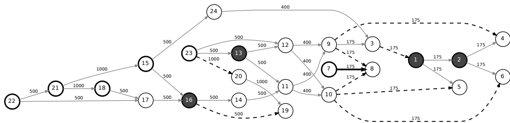
Figure 6.10: IEEE RTS-24 oriented by DC power flow at peak load. Edge labels are line ratings in MVA; double-circuit pairs are one edge with the summed rating. Bold outlines mark the eleven generator buses, and filled nodes mark the four generators (buses 1, 2, 13 and 16) that are at their nameplate limit in the maximum flow found under the net-injection model. The bold line 7–8 has 4 MVA of headroom, the least of any line. Dashed lines form the nine-line binding cut of the structural-subset model, which is a transmission bottleneck only when the mixed buses are excluded from supply and demand.
